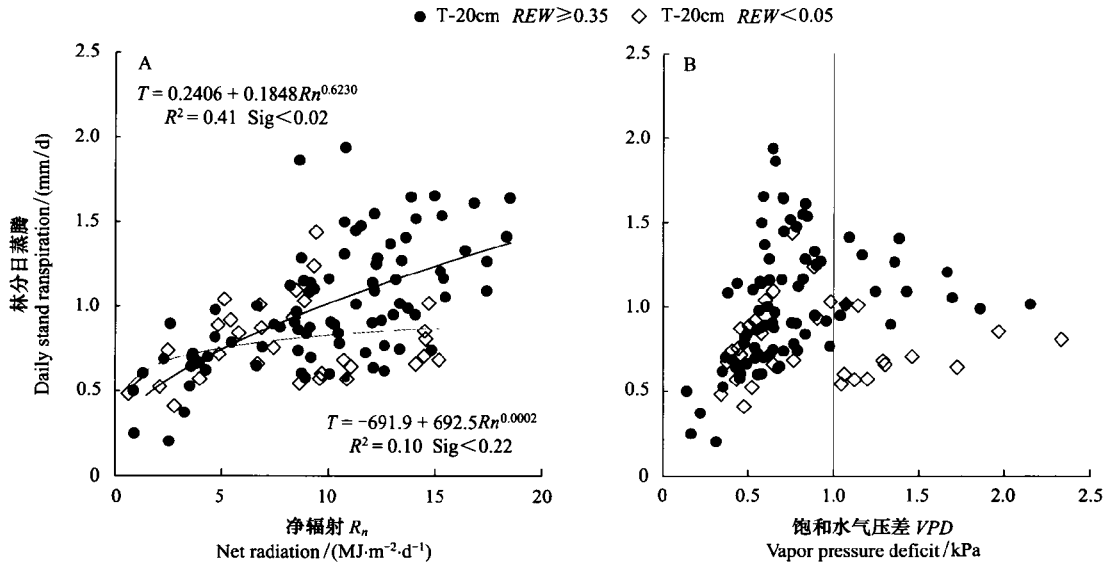
图 5 林分日蒸腾与净辐射、饱和水汽压的关系 Fig.5 The relationships between daily stand transpiration and R_n , VPD
